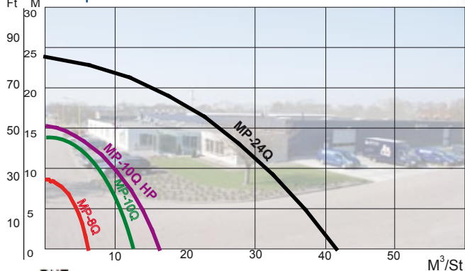
Pump Characteristics
